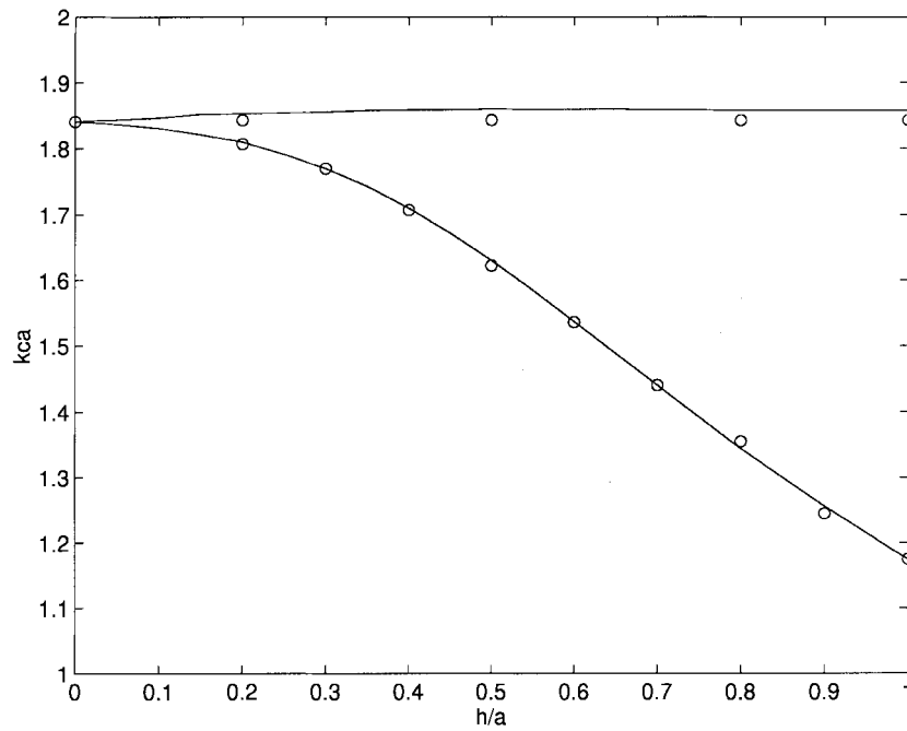
Fig. 4. Cutoff wavenumber of a ridged circular waveguide as a function of h/a when \theta = 2.29^\circ . The circles are from [9].
