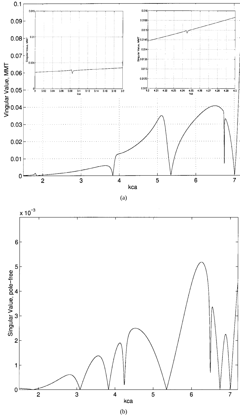
Fig. 3. Minimum singular value of [A(ka)] as a function of ka when h/a = 0.9 , \theta = 2.29^\circ , and M = N = 6 . (a) Standard MFMT and (b) pole-free MFMT.
