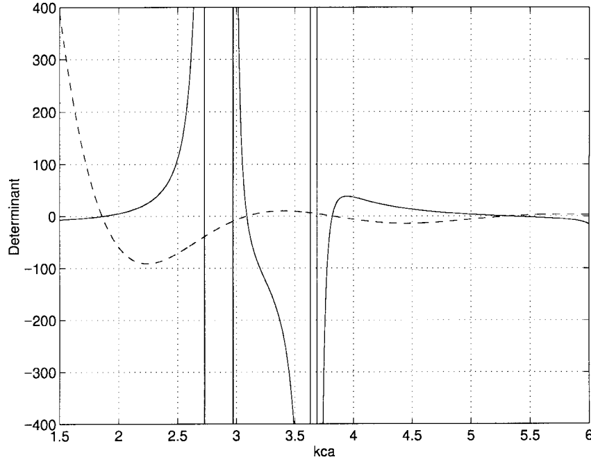
Fig. 2. Determinant of [A(k_c)] as a function of k_c a when h/a = 0.5 , \theta = 2.29^\circ , and M = N = 3 from the standard MFMT (solid line) and the pole-free MFMT (dashed line).
